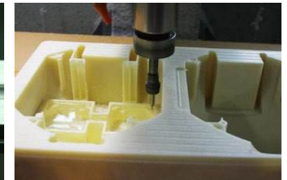
ABS Processing
